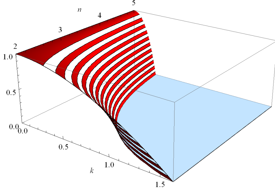
Figure 4.1: Profit improvements over the efficient auction \frac{\Pi^* - \Pi^E}{\Pi^M - \Pi^E} .
